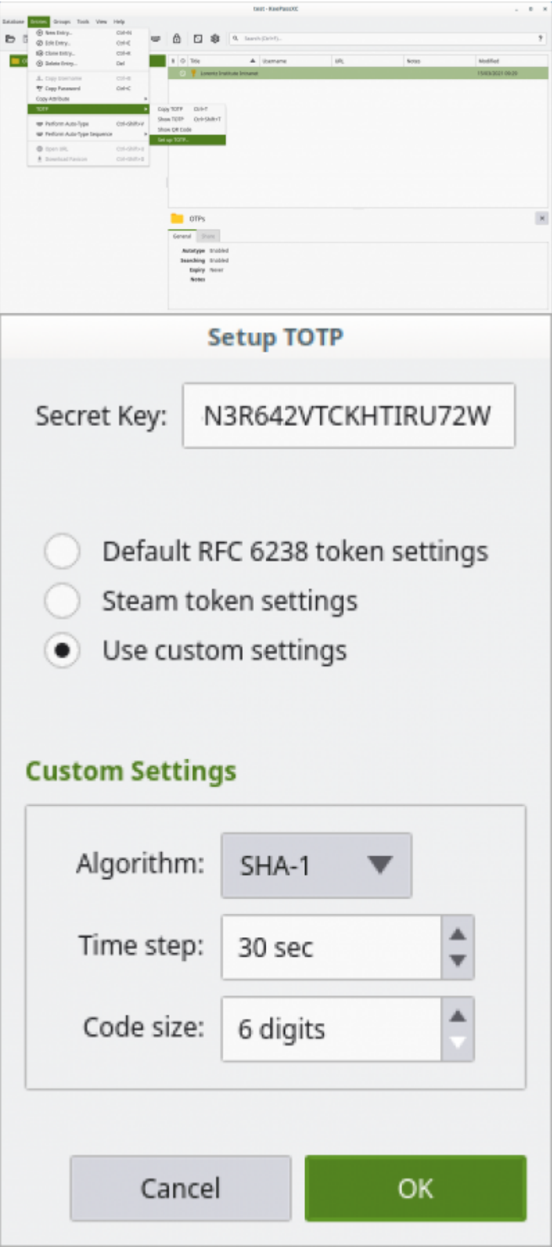
Figure 3: TOTP Setup with KeePassXC
