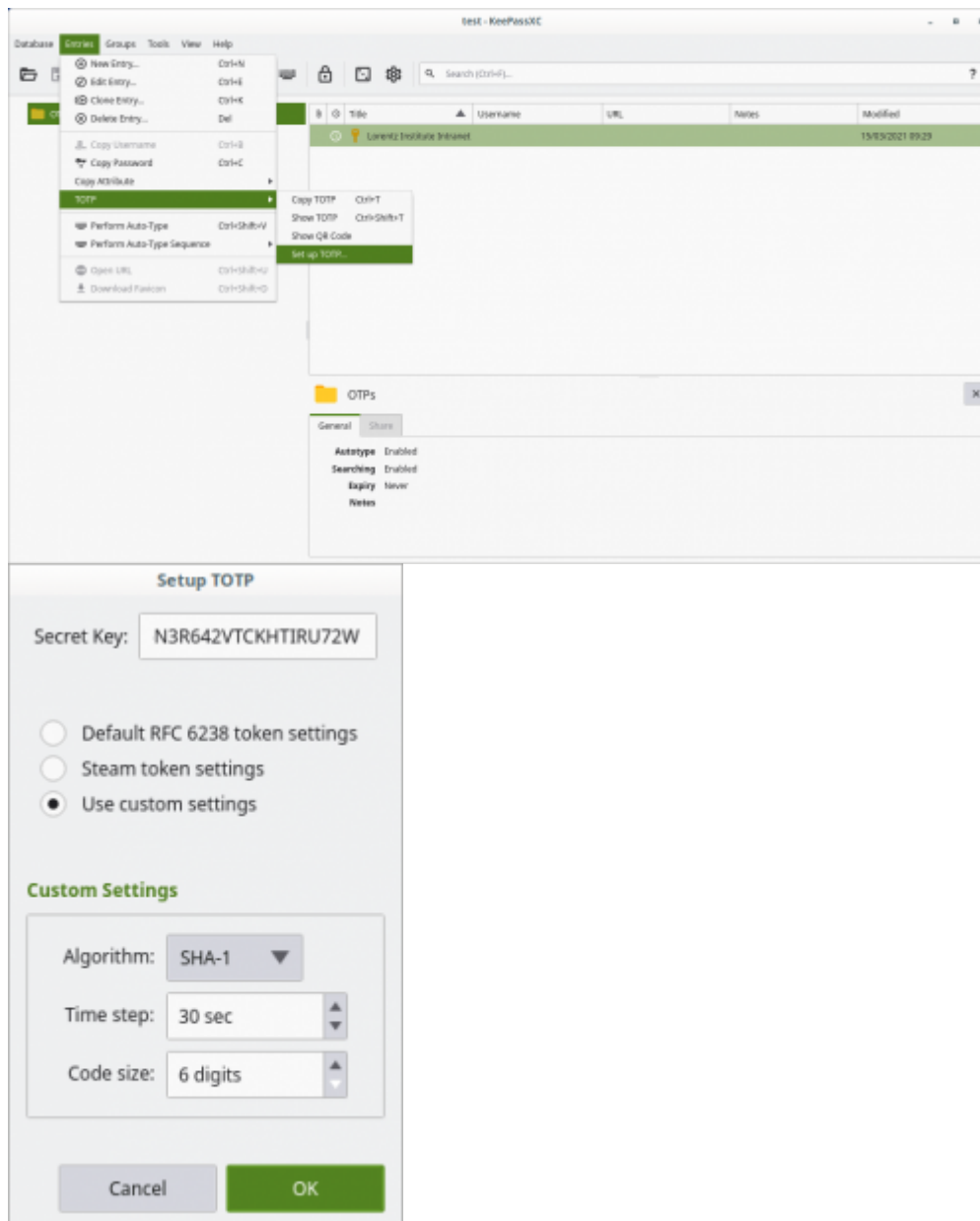
Figure 3: TOTP Setup with KeePassXC
